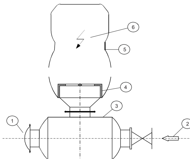
Figure 1 : Test rig for flashback test
