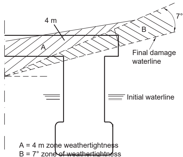
Figure 4 : Residual damage stability requirements for column stabilized units (1/1/2013)
