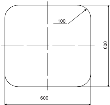
Figure 7 : Minimum horizontal hatch size (1/7/2011)
