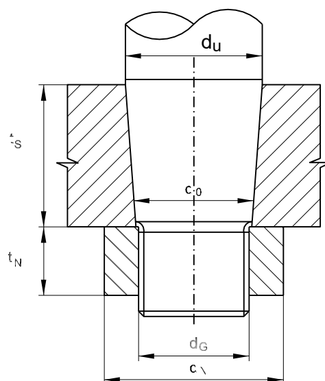
Figure 2 : Geometrical of cone coupling
