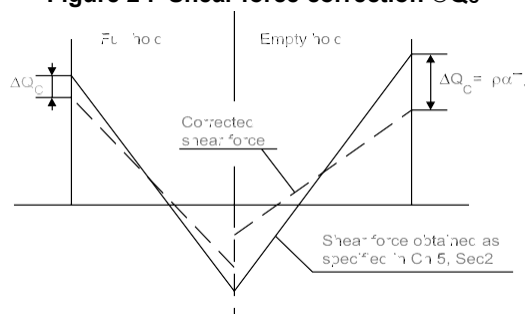
Figure 2 : Shear force correction \otimes Q_c
