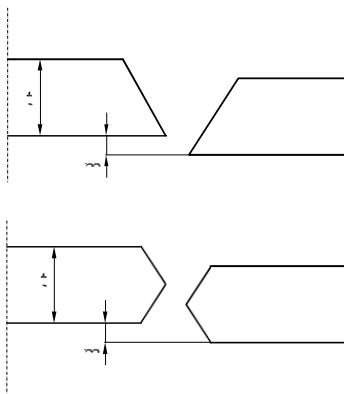
Figure 12 : Plate misalignment in butt connections
