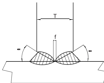
Figure 10 : Full penetration weld
