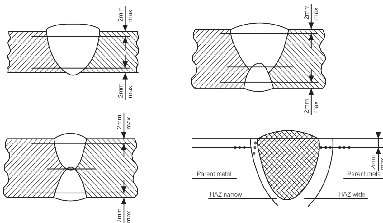
Figure 5 : Examples of hardness indentations (1/1/2007)
