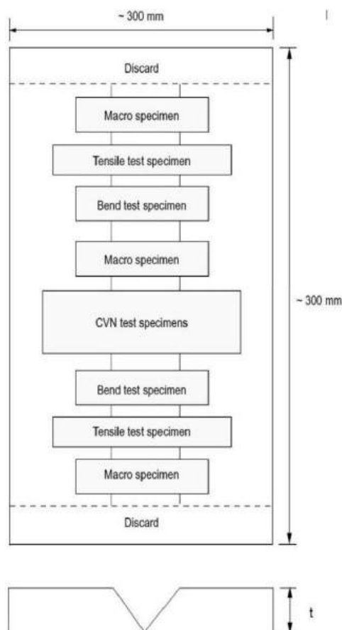
Figure 16 : Test Specimen for cast steel propellers (1/7/2021)
