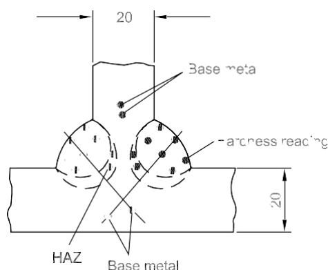
Figure 4 : Hardness readings (1/7/2019)
