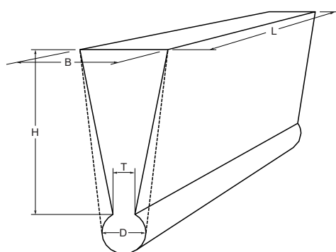
Figure 1 : Keel block test sample casting (1/1/2025)
