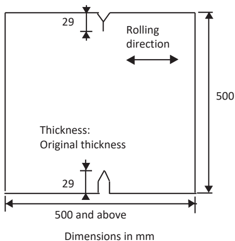
Figure 2 : Shape and size of specimen (1/1/2014)
