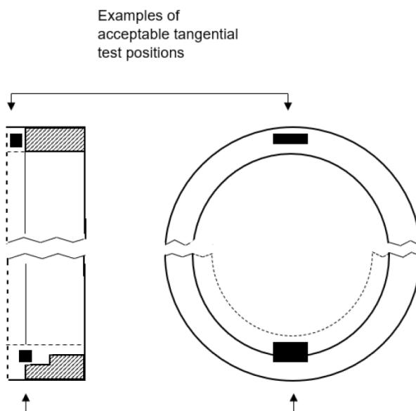
Figure 6 : Forged rings (1/7/2023)
