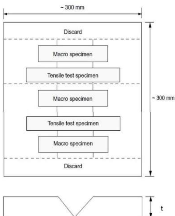
Figure 15 : Test Specimen for cast copper alloy propellers (1/7/2021)
