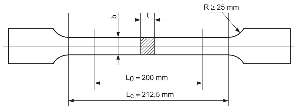
Figure 2 : Non proportional flat specimen (1/7/2004)
