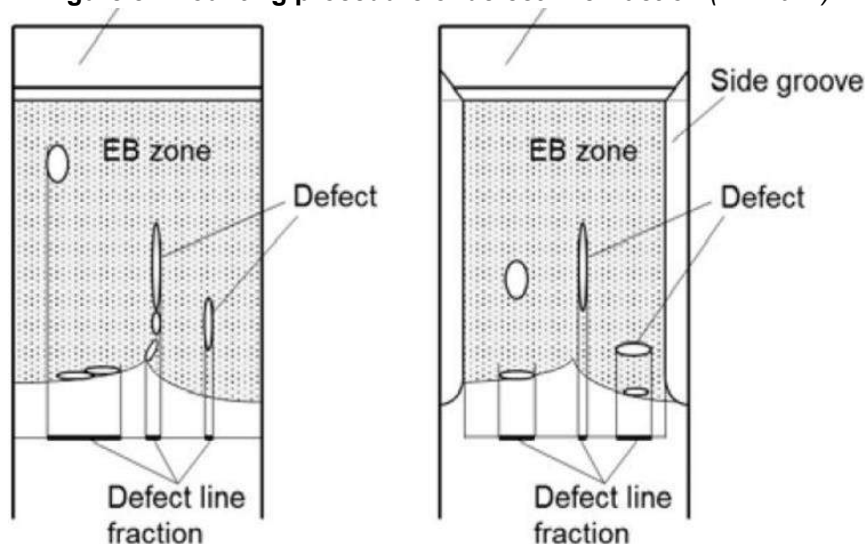
Figure 8 : Counting procedure of defect line fraction (1/1/2021)
