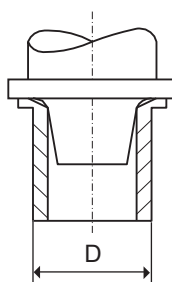
Figure 11 : Flanging test (1/7/2004)
