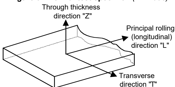
Figure 9 : Normal test specimen (1/7/2003)
