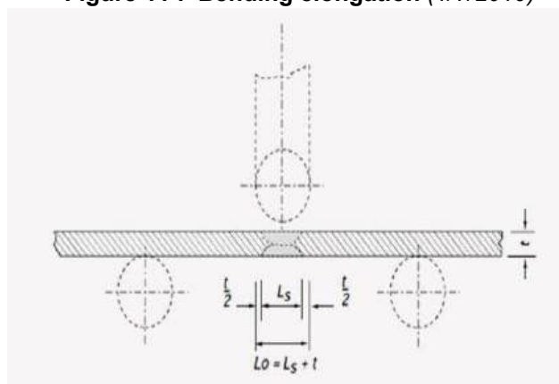
Figure 11 : Bending elongation (1/7/2019)
