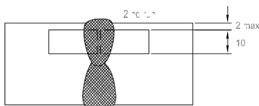
Figure 8 : Charpy V-notch impact test specimens (1/7/2019)
