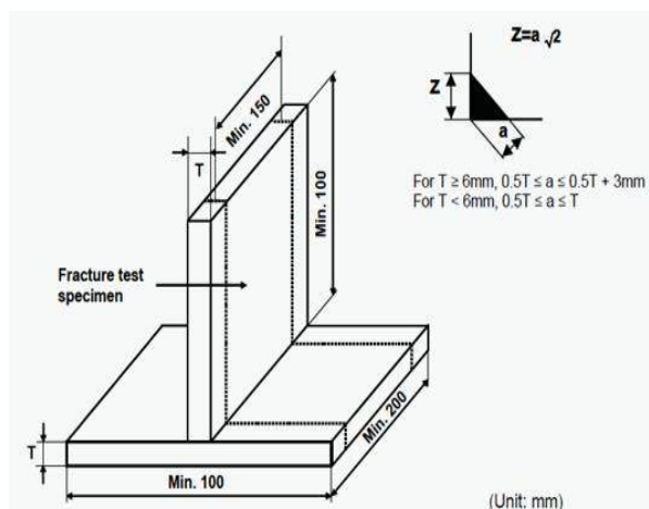
Figure 5 : Dimensions and types of test assembly for tack butt welds (1/1/2018)
