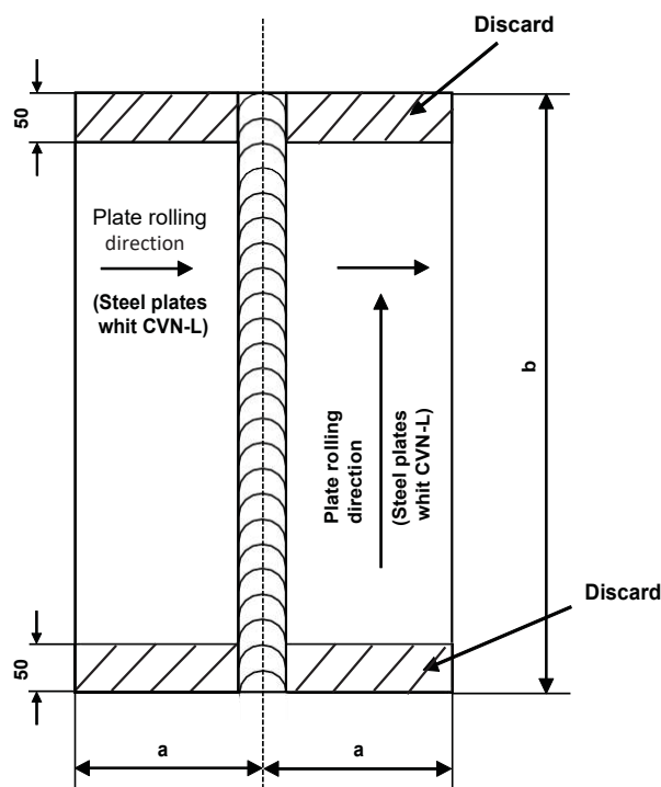
Figure 1 : Plate butt weld test assembly (1/1/2015)
