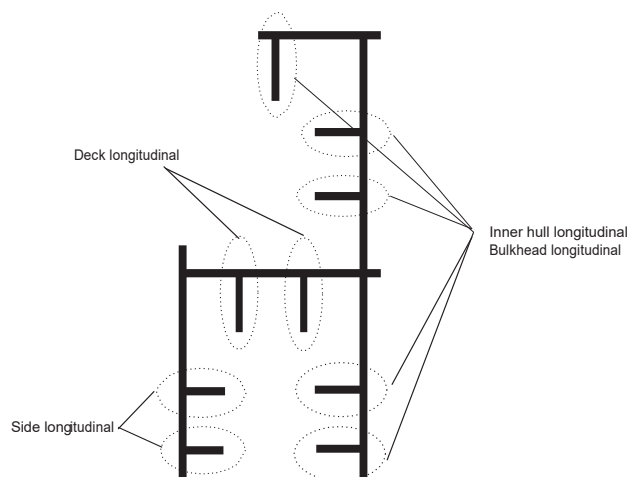
Figure 12 : Upper flange longitudinal structural members (1/1/2014)
