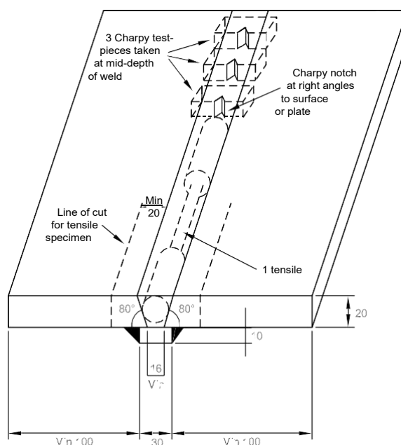
Figure 1 : Deposited metal test assembly (1/7/2019)
