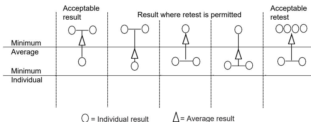
Figure 11 : Diagram showing acceptance / rejection and retest criteria (1/7/2003)
