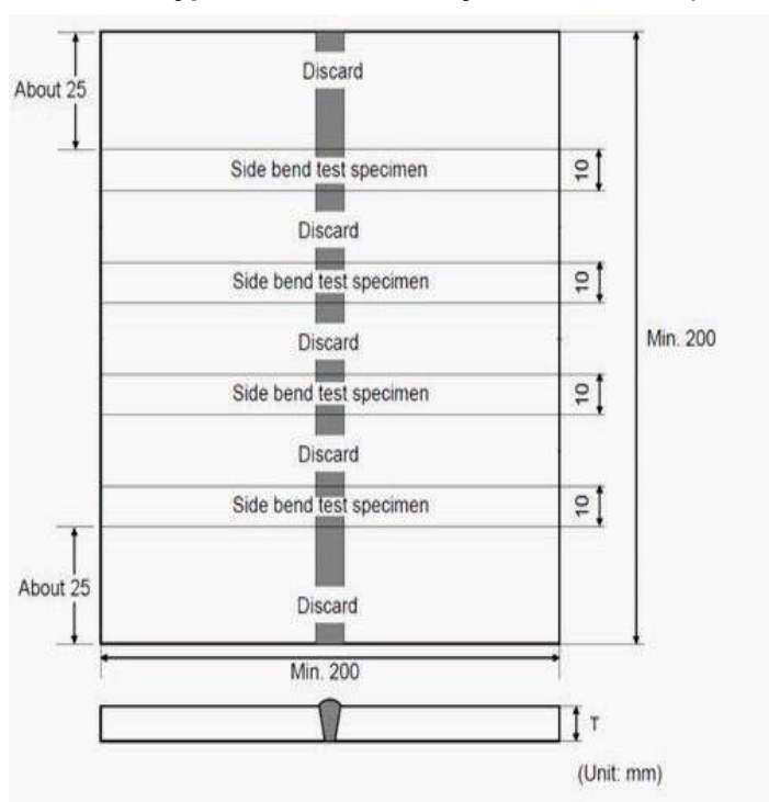
Figure 3 : Dimensions and types of test assembly for butt welds ( T > 12\text{mm} ) (1/1/2018)
