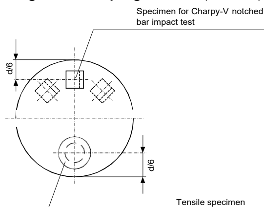
Figure 3 : Sampling locations (1/7/2003)
