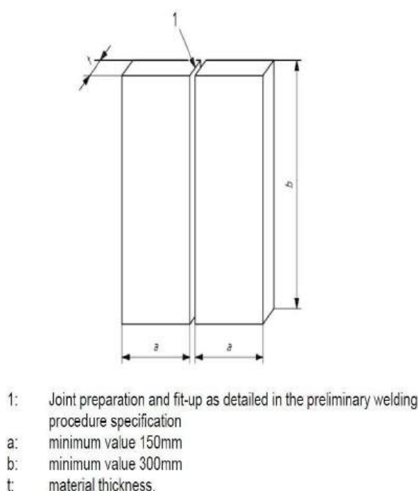
Figure 14 : Test piece for welding repair procedure for cast copper alloy propellers and cast steel propellers (1/1/2025)
