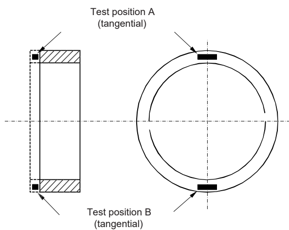
Figure 9 : Gear wheel rim made by expanding
