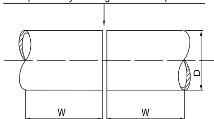
Figure 10 : Pipe weld test assembly
