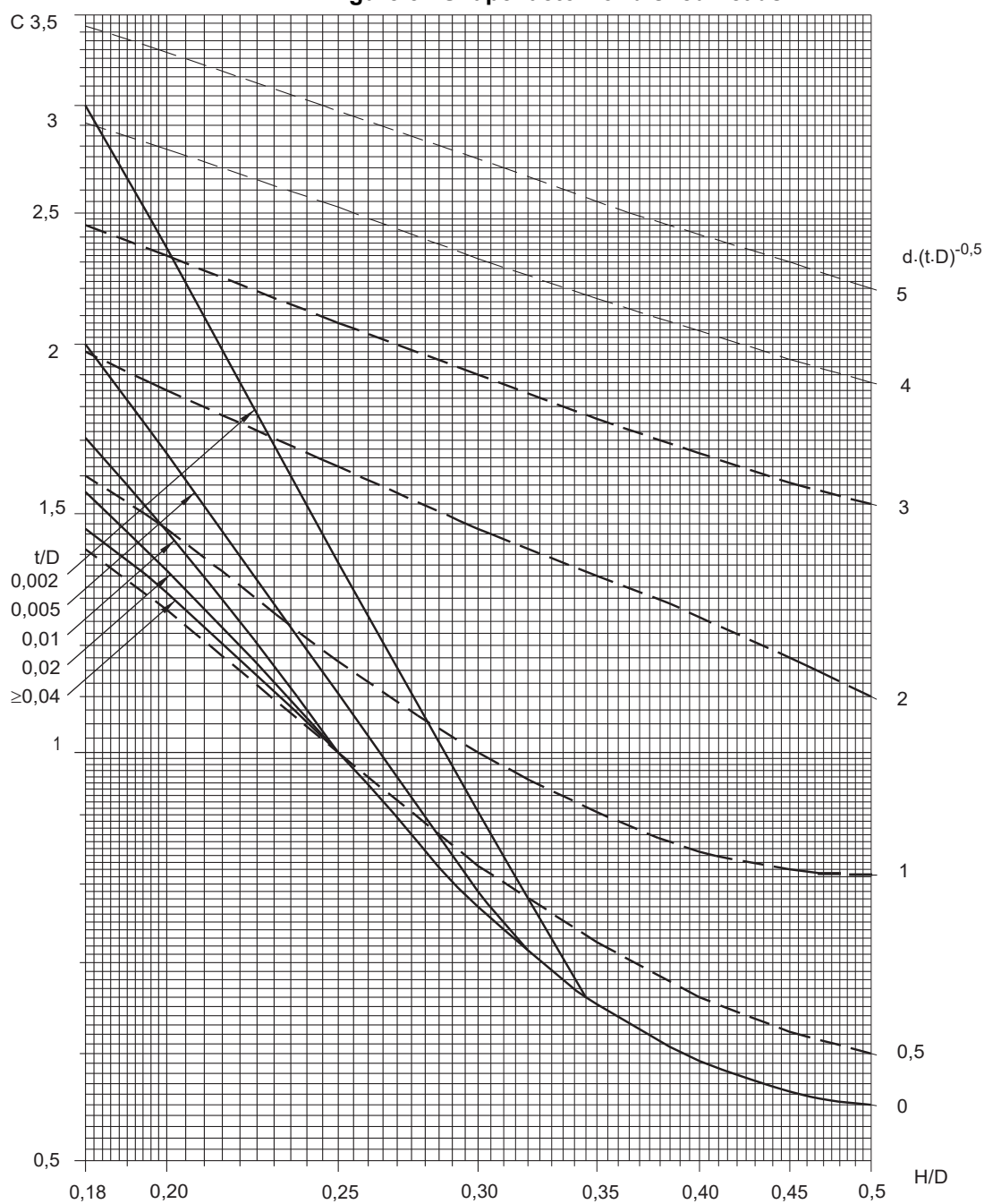
Figure 6 : Composed torispherical head (1/7/2001)
