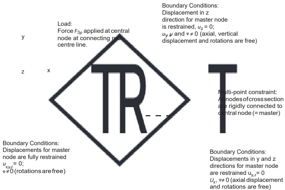
Figure 9 : Boundary and load conditions for the 3-point bending load case of an in-line engine (1/1/2012)
