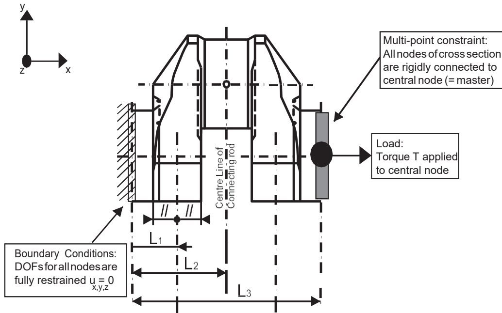
Figure 7 : Boundary and load conditions for the torsion load case (1/1/2012)
