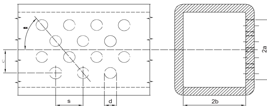
Figure 13 : Rectangular section headers
