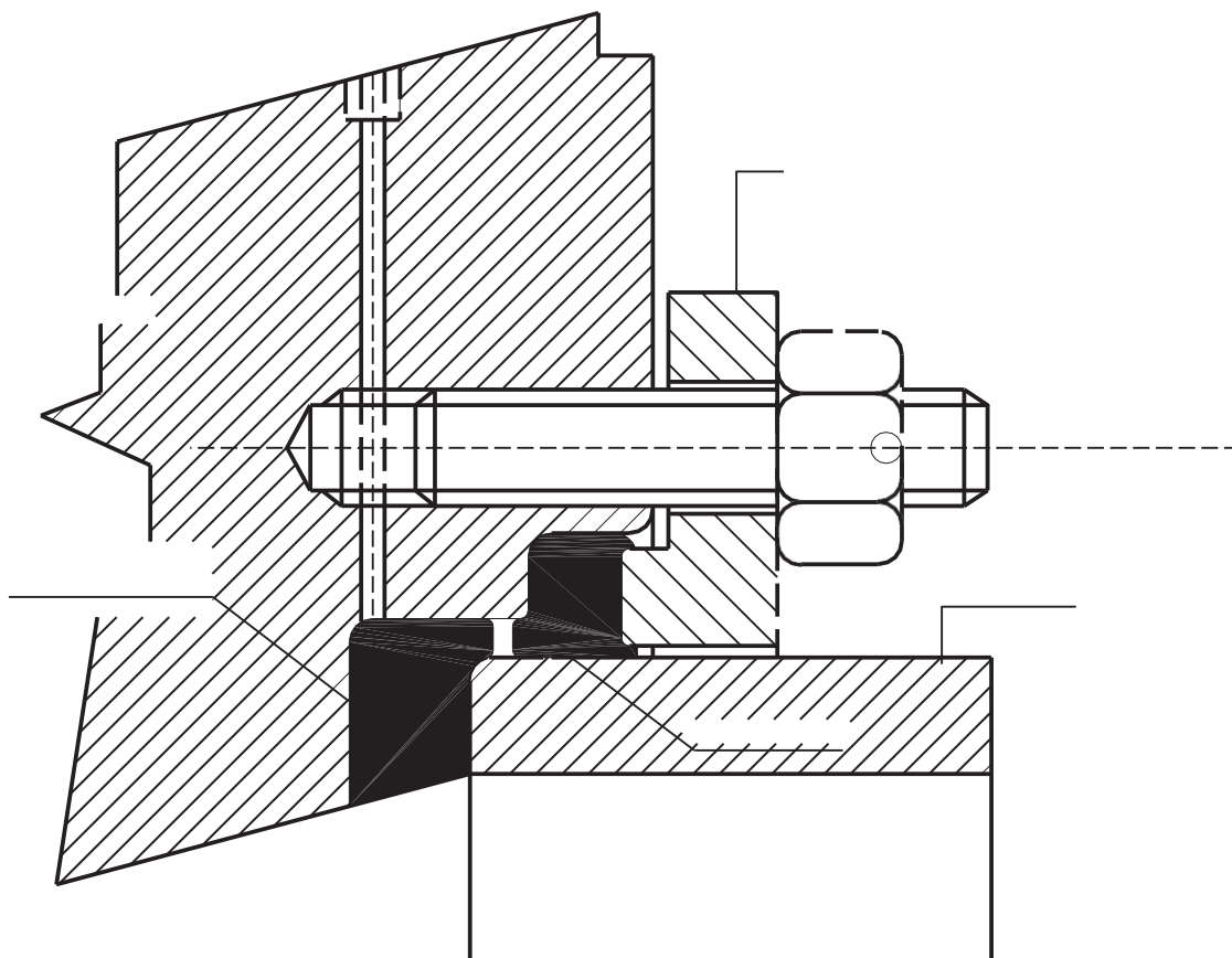
Figure 2 : Example of sealing arrangement
