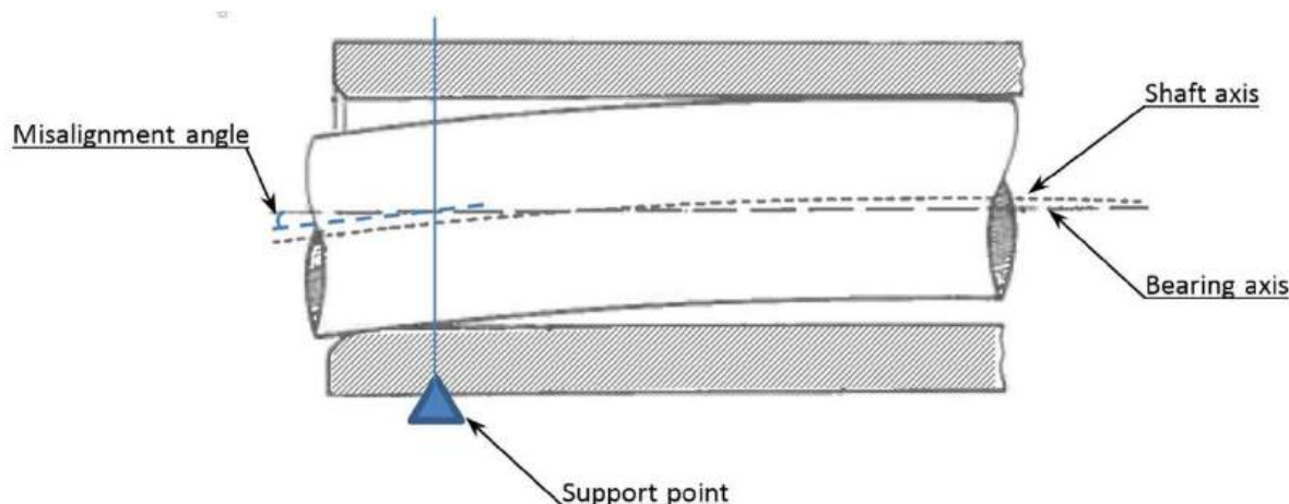
Figure 2 : Misalignment angle (15/2/2024)
