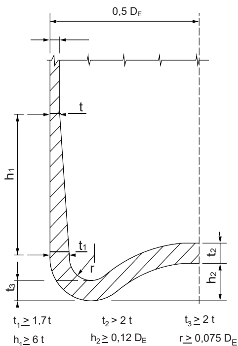
Figure 18 : Heads with openings
