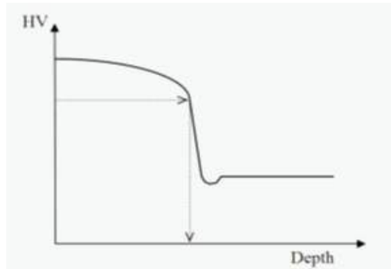
Figure 20 : Typical hardness as a function of depth. The arrows indicate the defined hardening depth. Note the indicated potential hardness drop at the transition to the core. This can be a weak point as local strength may be reduced and tensile residual stresses may occur (1/7/2018)
