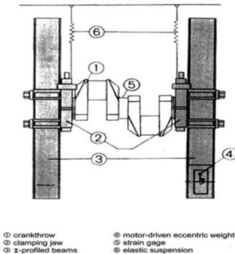
Figure 15 : Example of testing arrangement of the resonance tester for torsion loading with double crank throw section (1/7/2018)
