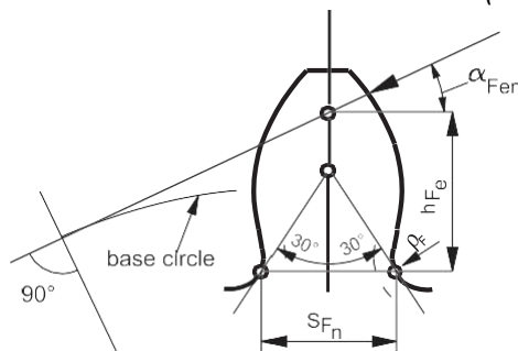
Figure 1 : Geometric elements of teeth (1/1/2001)
