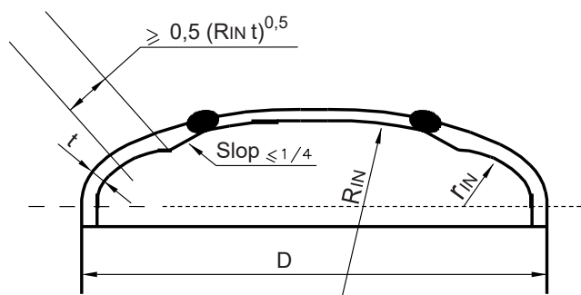
Figure 6 : Composed torispherical head (1/7/2001)
