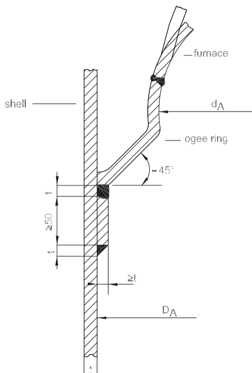
Figure 15 : Ogee Ring
