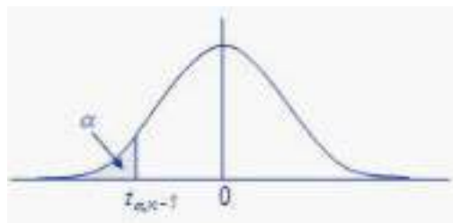
Figure 11 : Student's t-distribution (1/7/2018)
