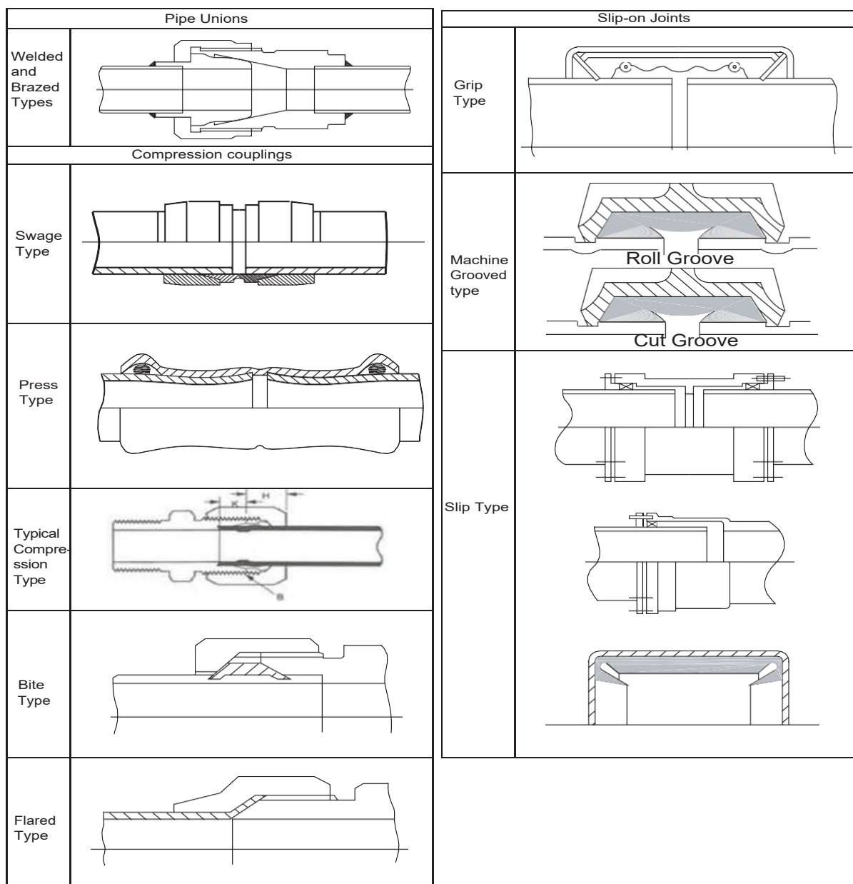
Figure 2 : Examples of mechanical joints (1/1/2020)
