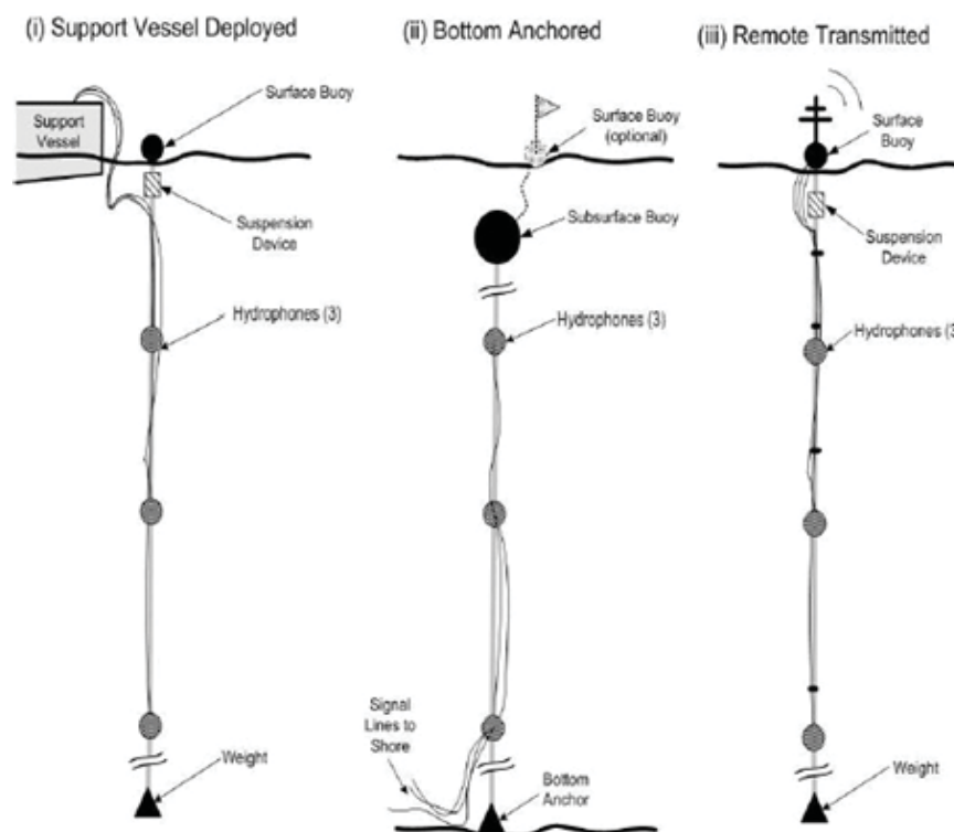
Figure 2 : Typical hydrophones deployment configurations (not to scale) (1/3/2008)
