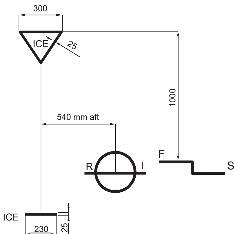
Figure 1 : Warning triangle (1/7/2007)
