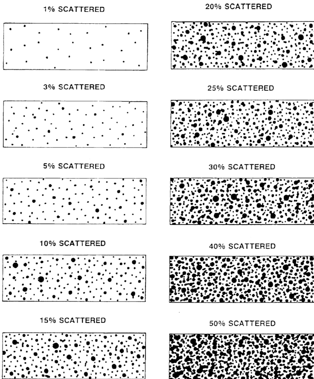
Figure 1 : Pitting intensity diagrams ( from 1% to 50% intensity)
