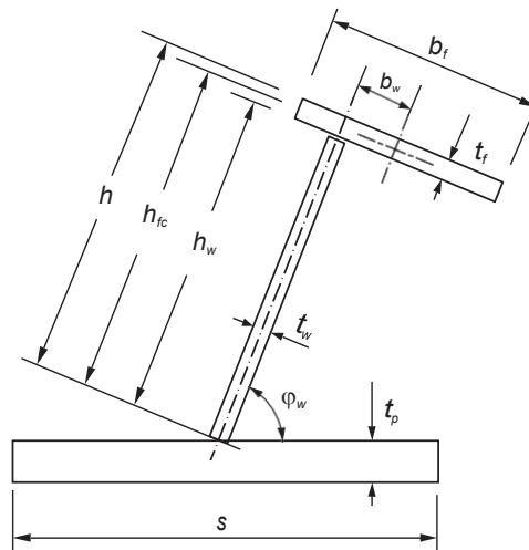
Figure 7 : Stiffener geometry (1/3/2008)
