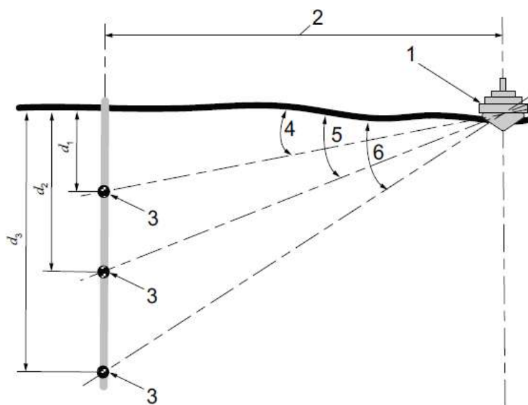
Figure 1 : Hydrophones geometry (1/1/2022)
