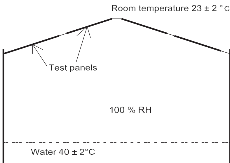
Figure 3 : Condensation chamber (1/7/2006)
