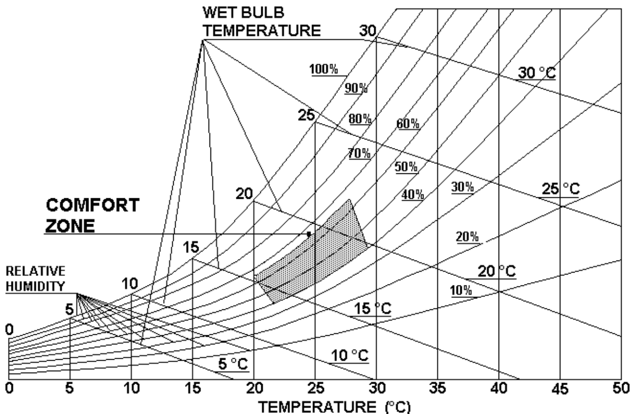
Figure 1 : Psychrometric chart
