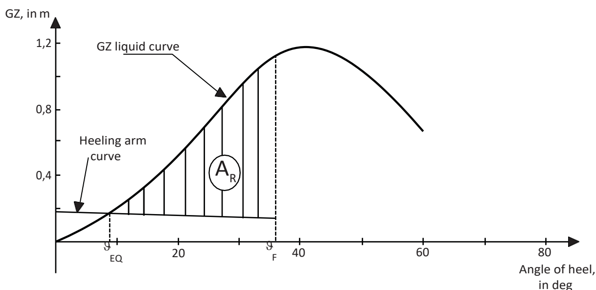
Figure 1 : Stability criteria (1/8/2011)
