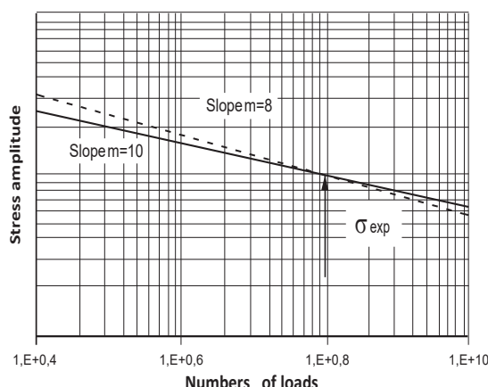
Figure 6 : Constant-slope S-N curve (1/7/2024)
