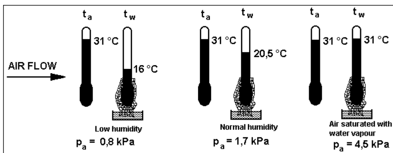
Figure 4 : Principle of operation of a psychrometer
