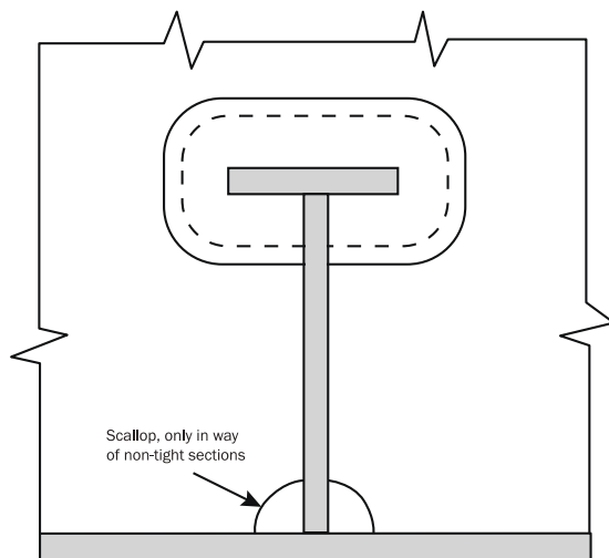
Figure 8 : Complete collar
