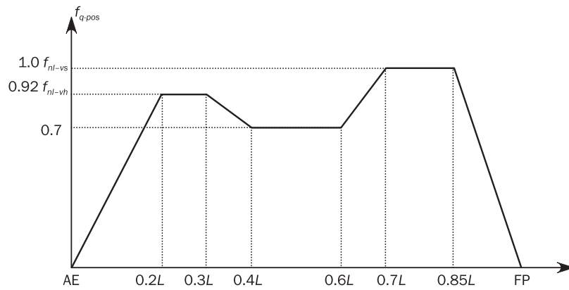
Figure 3 : Distribution factor of positive vertical shear force f_{q-pos}
