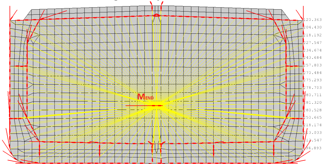
Figure 10: Adjustment loads
