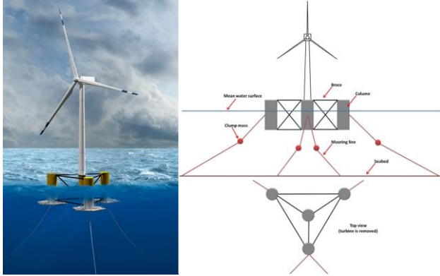
Fig 7: Semi-submersible concept
