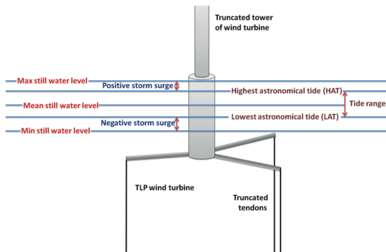
Figure 3: water level definitions
