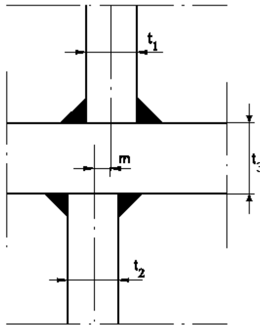
Figure 56: Cruciform connection
