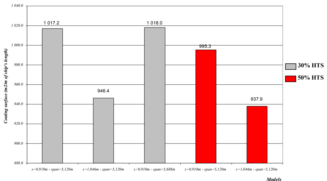
Figure 38: Midship section coating surfaces.
