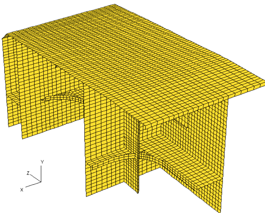
Figure 7: “Fine mesh” finite element model of a stringer detail.
