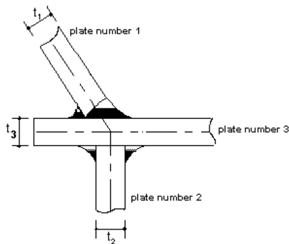
Figure 55: Angle connection
