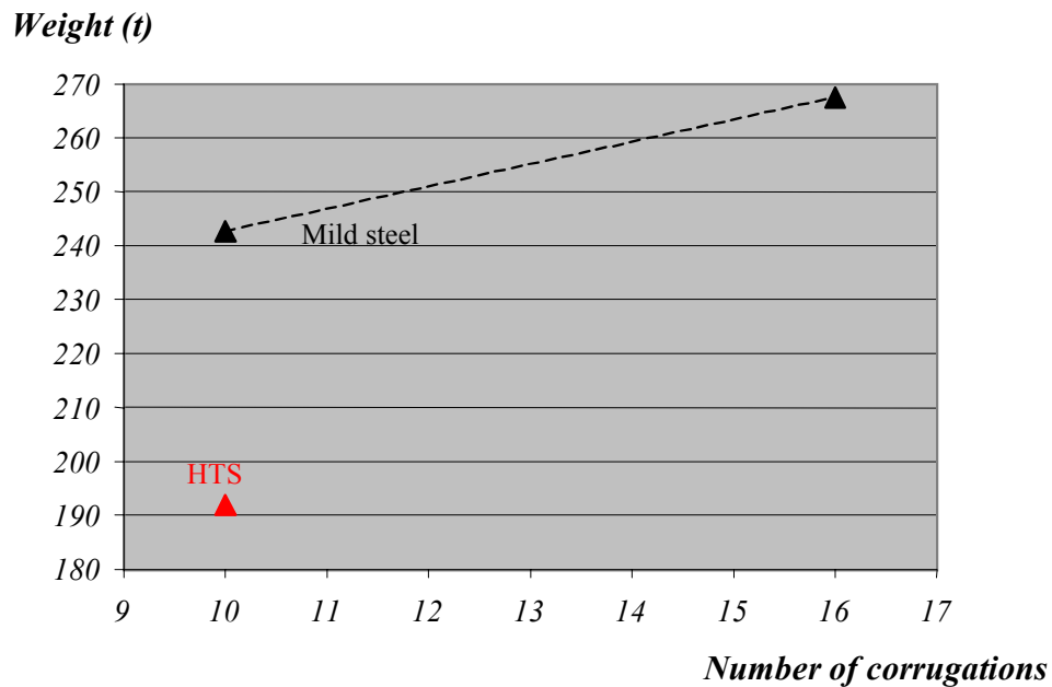
Figure 31: Influence of the number of corrugations on the corrugated bulkhead steel weight.
