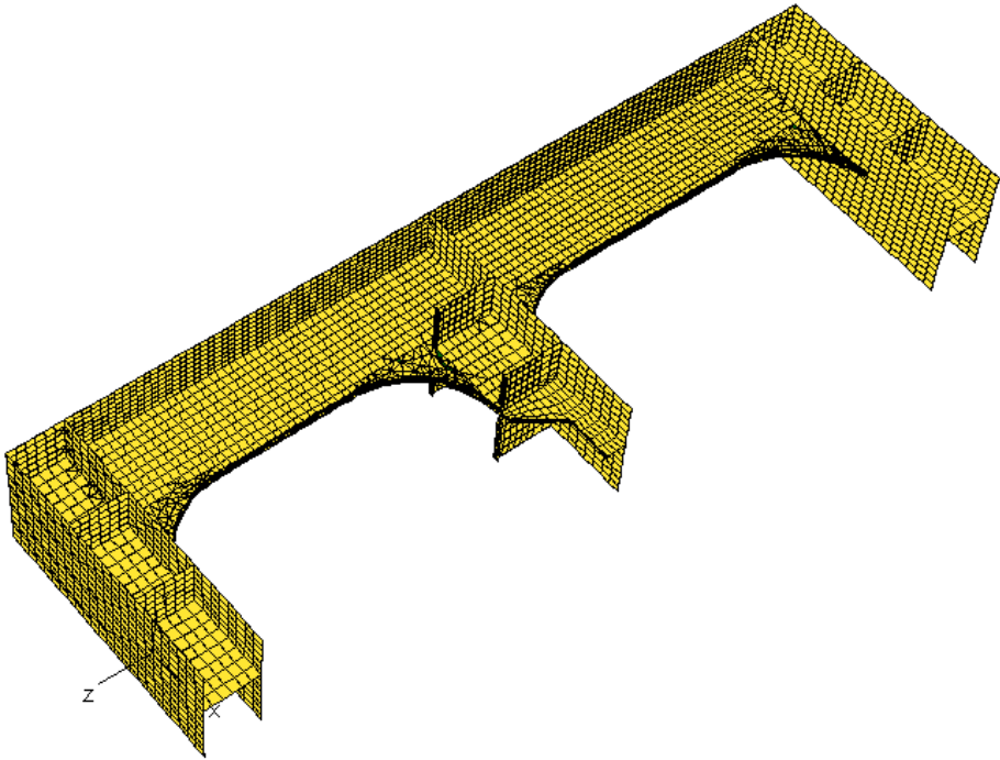
Fig. 6: “Fine mesh” finite element model of the upper transverse bulkhead stringer.
