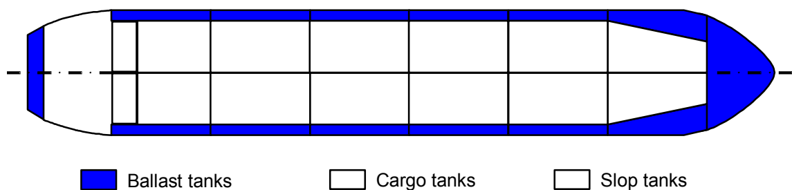
Figure 1: Cargo and ballast tank arrangement for tankers up to Suezmax size.
