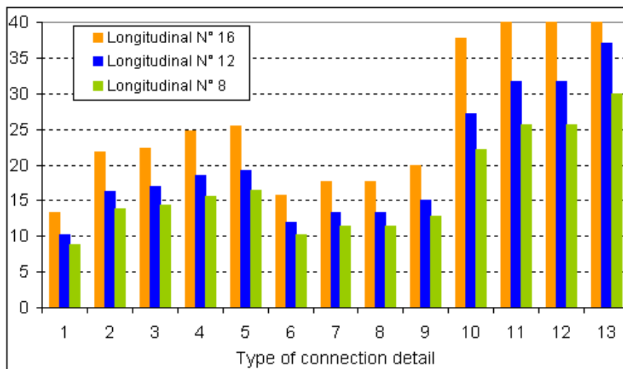
Figure 64: Fatigue life, in years, for different connection details – Side shell longitudinal stiffeners (ship SH#01).
