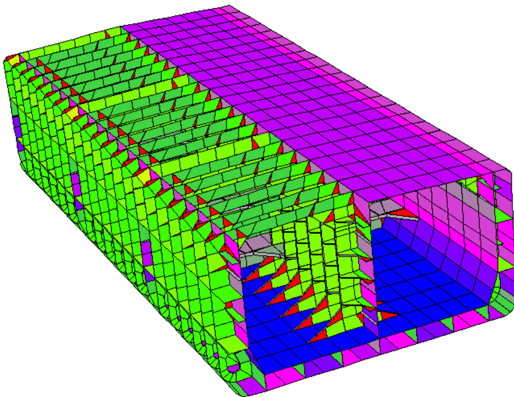
Fig. 1: Three cargo tank “coarse mesh” model (starboard deck plating and starboard side shell plating are removed for illustration purposes).
