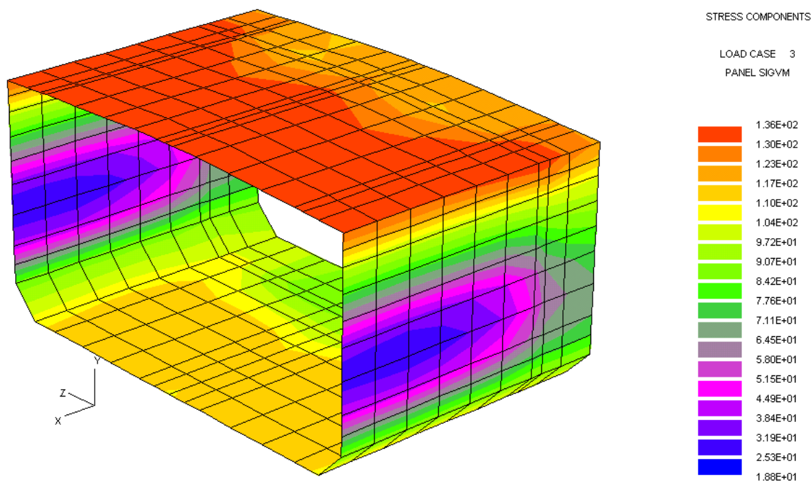
Figure 3: Maximum Von Mises stresses' results of the “coarse mesh” three cargo tank finite element analysis on the primary supporting members.
