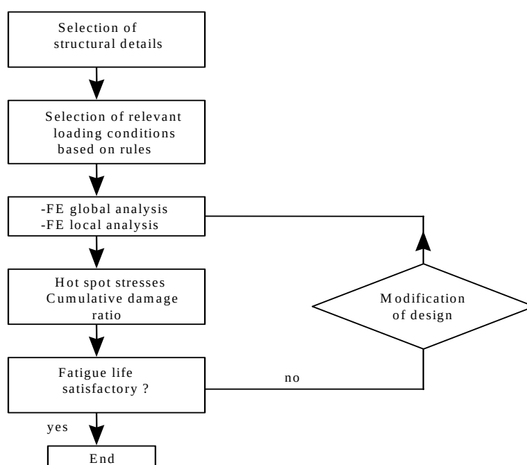
Figure 2.9: Fatigue Analysis
