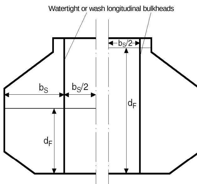
Figure 2.11: Example of tank designed to reduce the sloshing pressures on its boundaries
