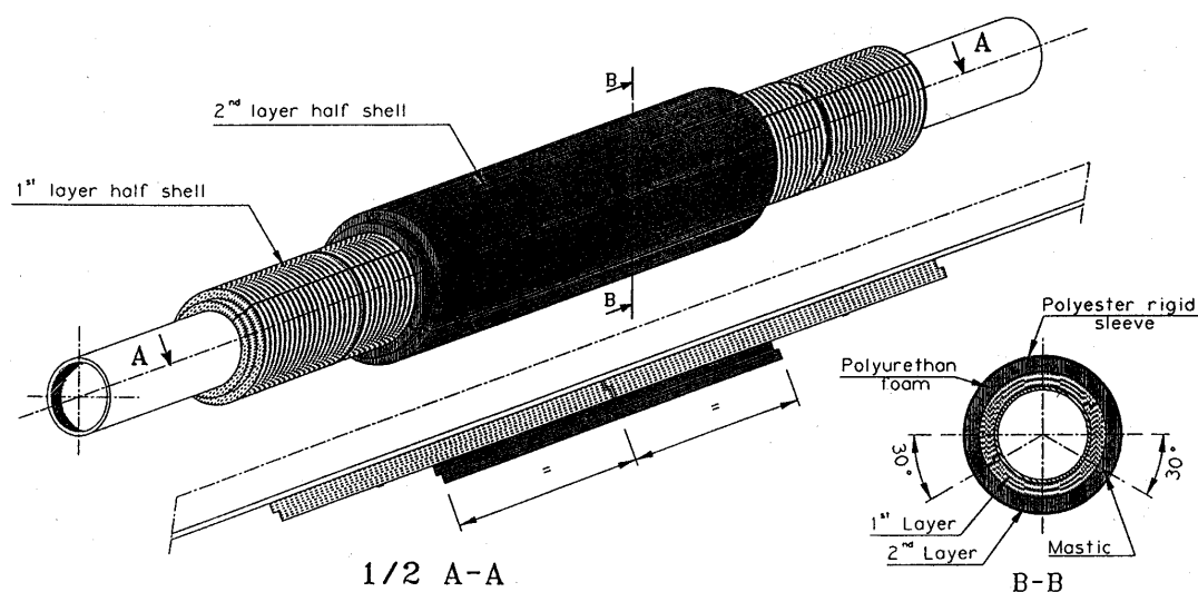
Pipe insulation principals
