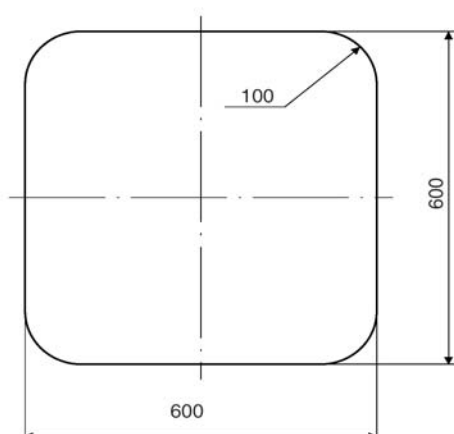
Figure 2.19: Minimum horizontal hatch size
