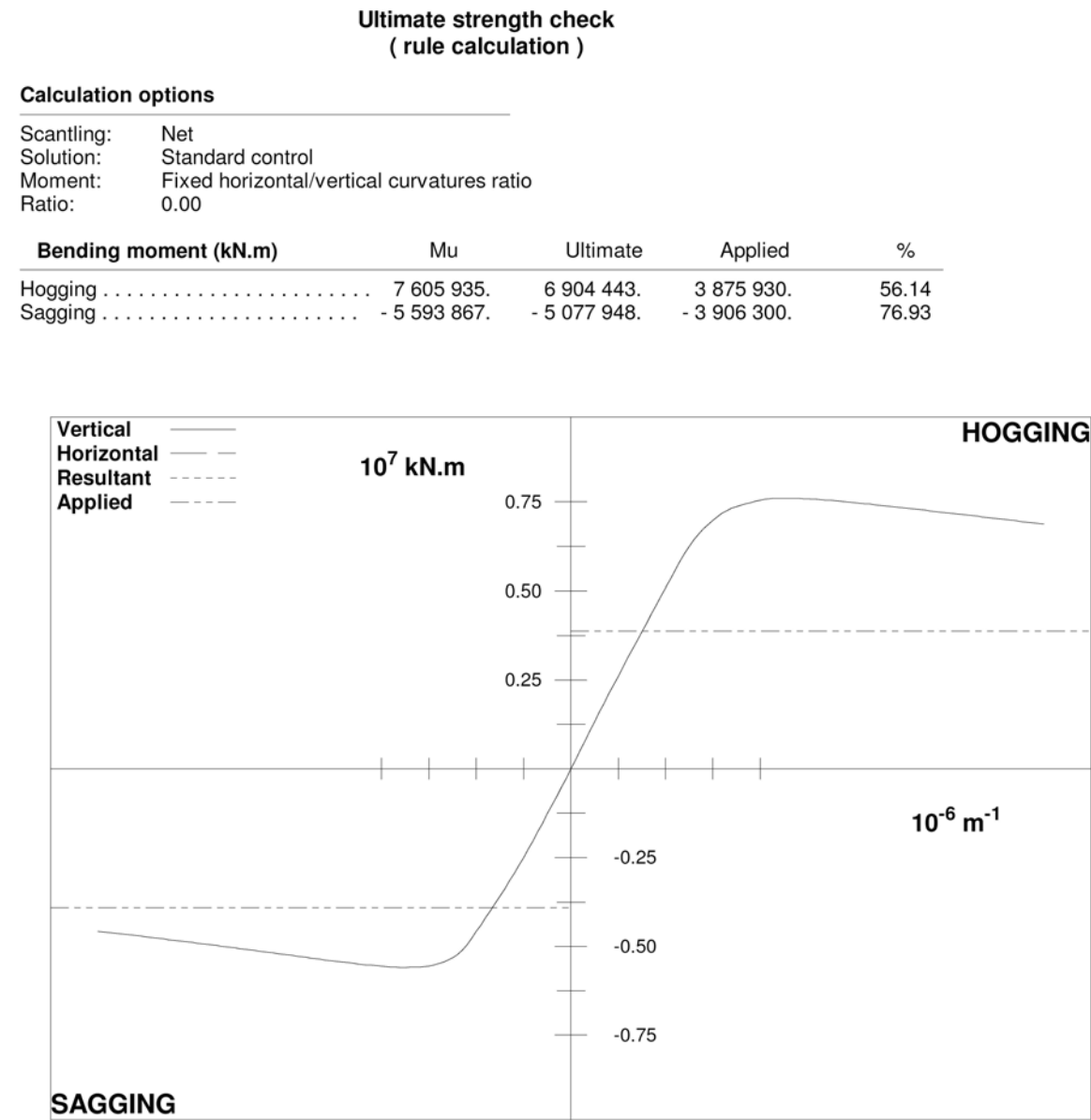
Figure 6.3: Hull girder ultimate strength check results
