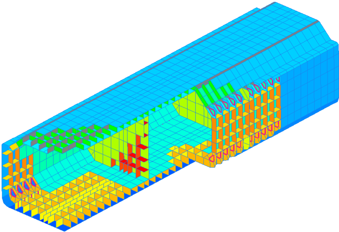
Figure 6.6: Global 3D structural model for the FEM analysis
