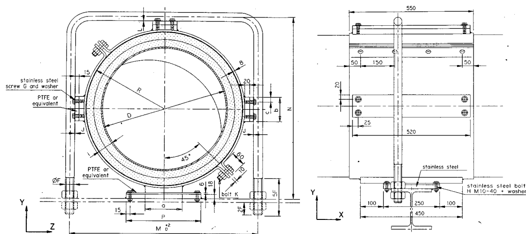
Figure 4.4: Pipe supports
