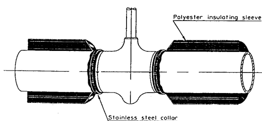
Singular points
