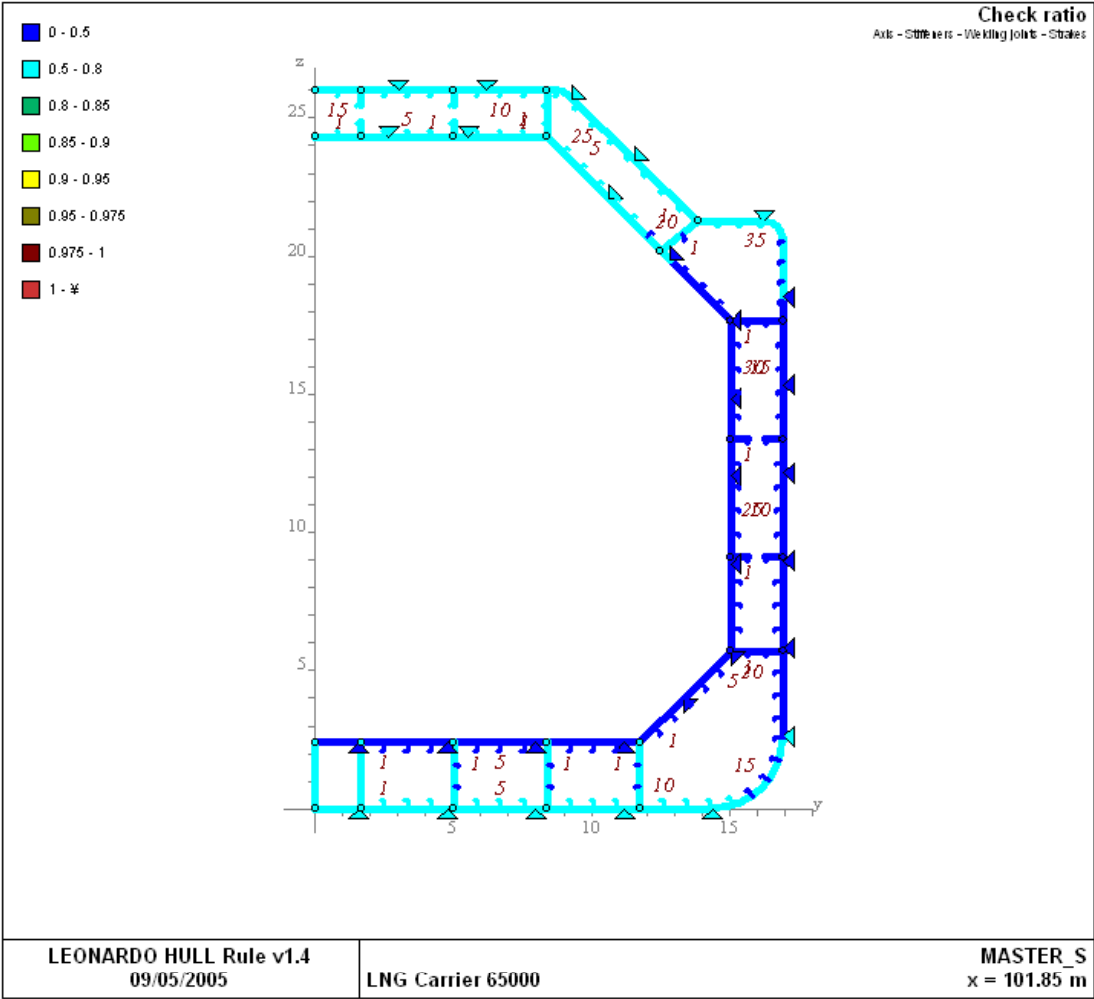
Figure 6.2: Hull girder yielding check results
