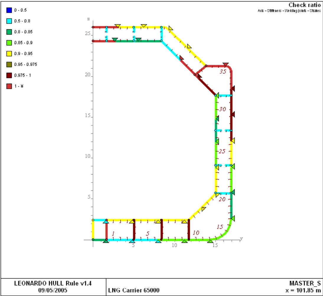
Figure 6.4: Plating strength check results
