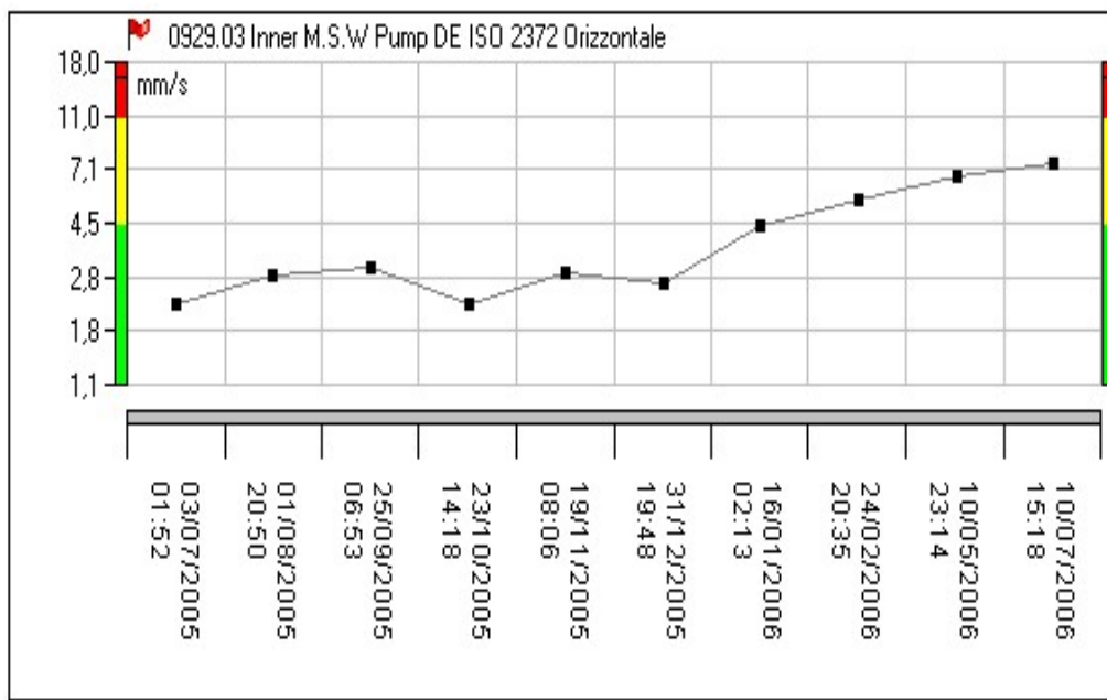
Figure 2: Typical plot of vibration readings
